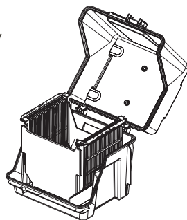
E124-60-101-69F02 box with K182-60MB-97C02 carrier
